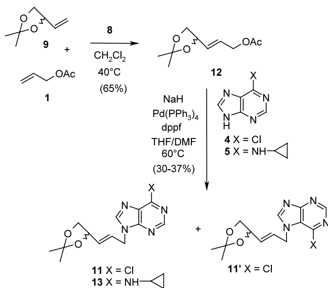
Scheme 2. Alternative synthesis of unsaturated purine acyclonucleosides 11 , 11' and 13 .
