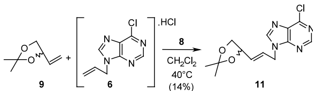
Scheme 1. Synthesis of acyclic nucleosides via cross-metathesis reaction in the purine series.
